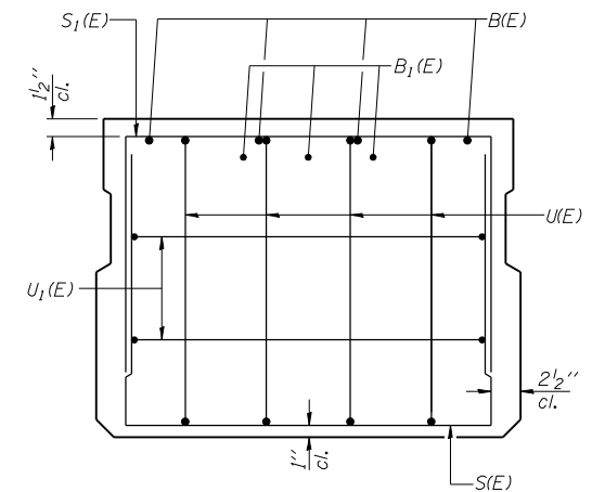
VIEW C-C
