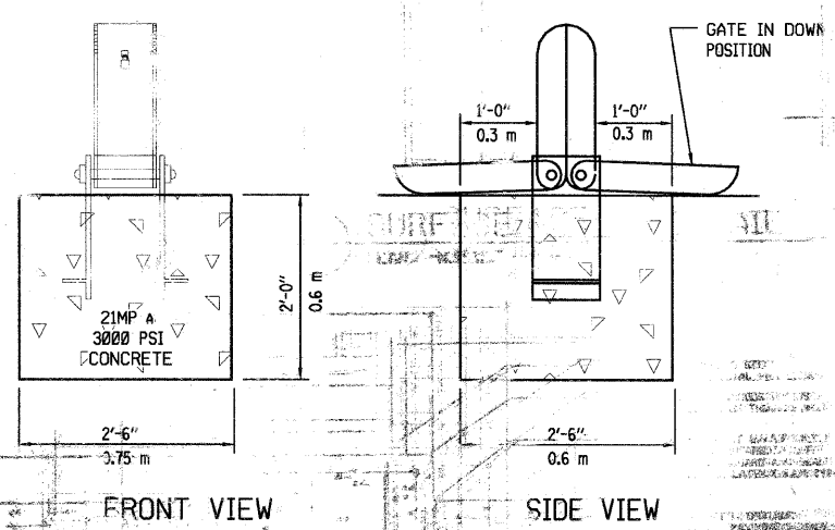
TIP DOWN GATE INSTALLATION DETAIL
