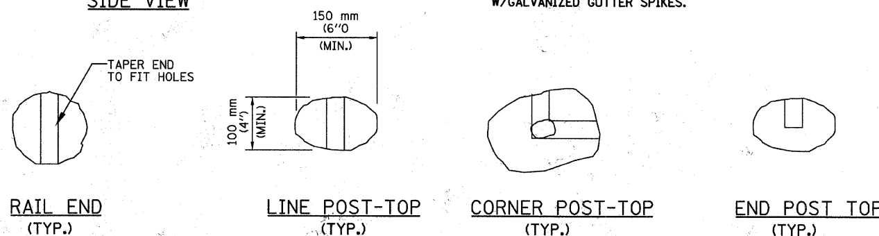
RUSTIC RAIL FENCE DETAIL
