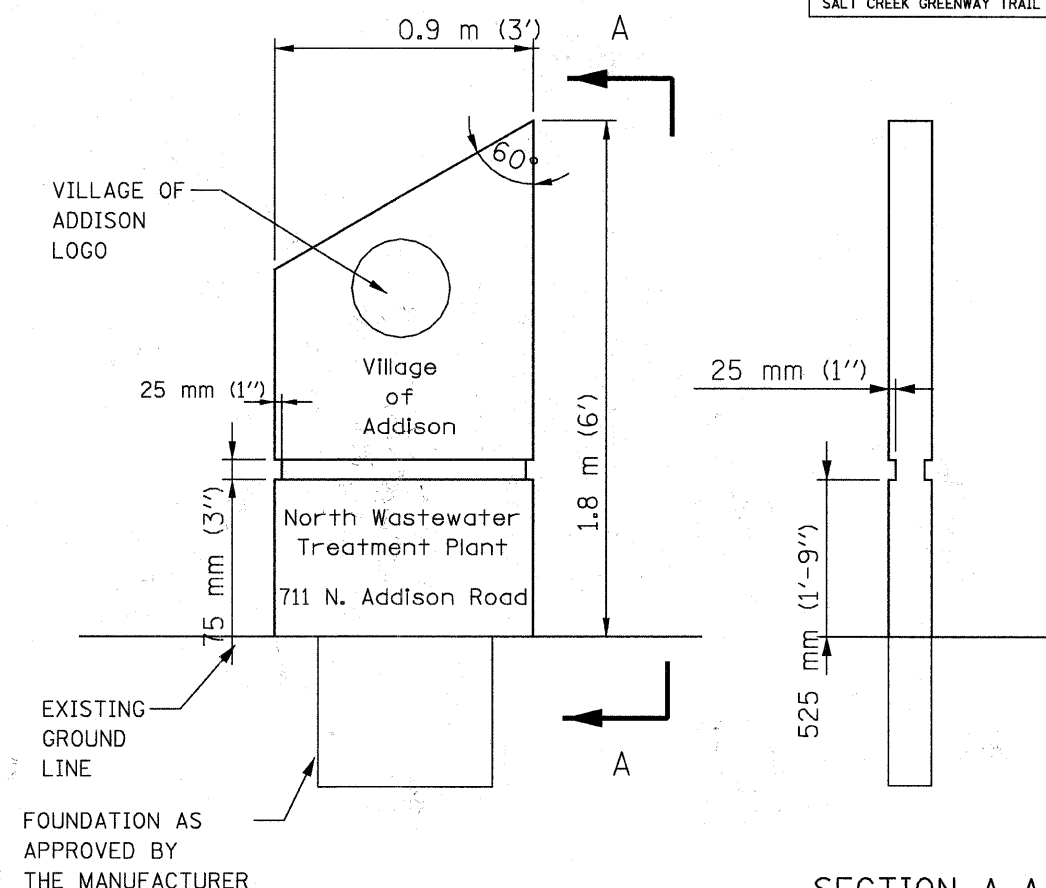
ENTRANCE MONUMENT DETAIL
