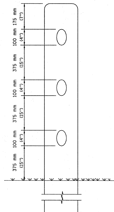
SIDE VIEW
