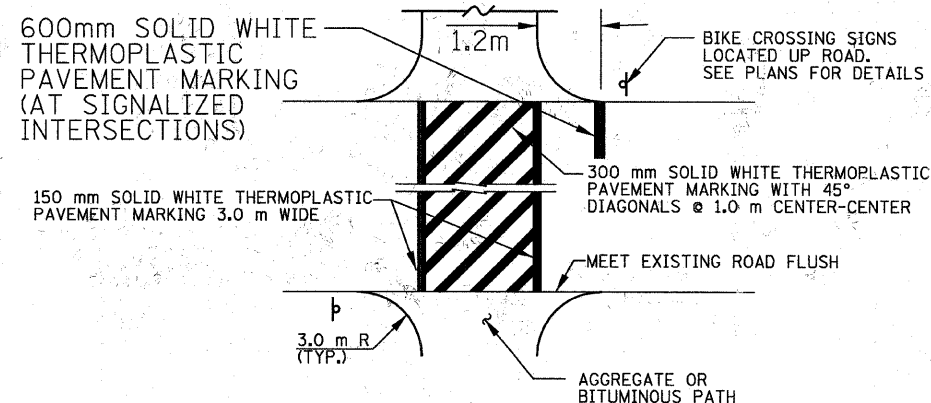
PAVEMENT MARKING DETAIL BICYCLE CROSSWALK MARKING
