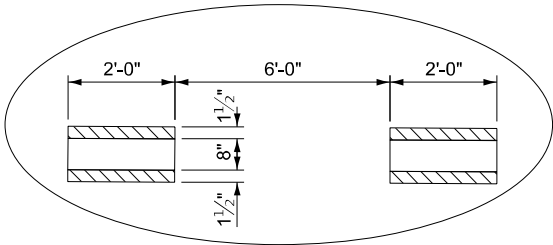
TYPICAL 8" LANE LINE (SKIP-DASH)
