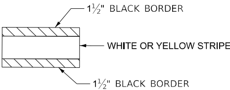
CONTRAST PAVEMENT MARKING DETAIL
