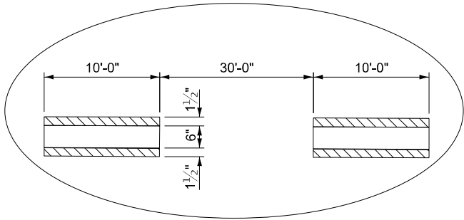
TYPICAL CENTERLINE STRIPING (SKIP-DASH)
