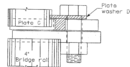
PLACEMENT OF PLATE WASHER D (PLAN)
