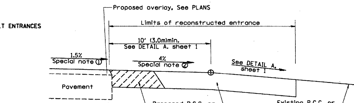
SECTION D-D RECONSTRUCTED P.C.C. OR HOT MIX ASPHALT ENTRANCE
