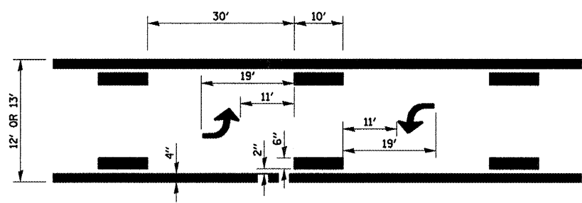
TYPICAL APPLICATION @ BI-DIRECTIONAL TURN LANE
