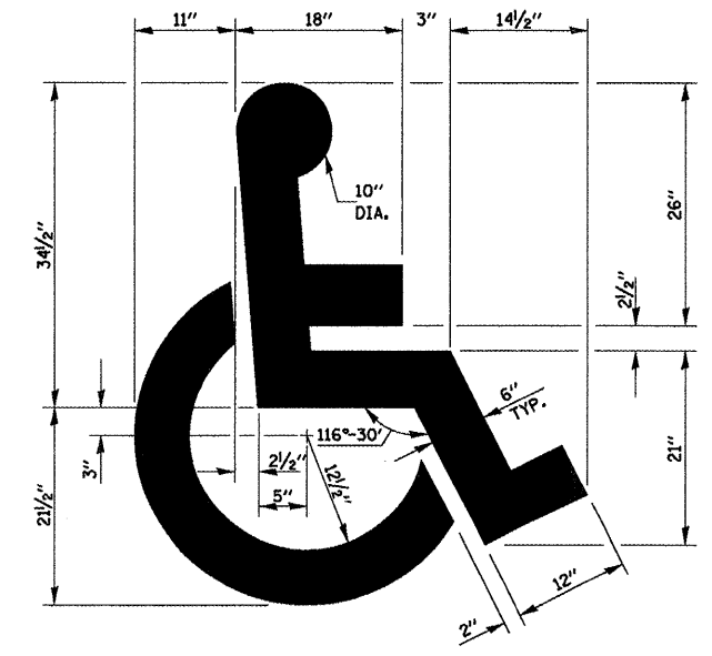
TYPICAL DETAIL FOR PAINTING HANDICAP MARKINGS
