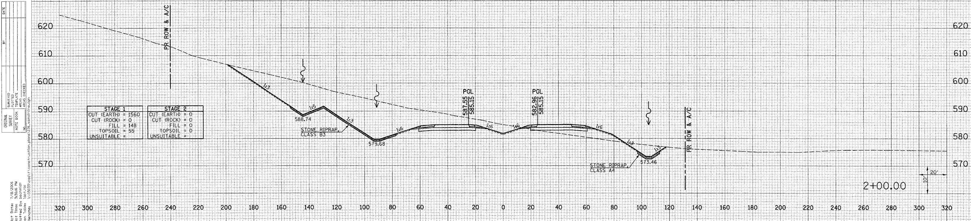
FAP ROUTE 315 (IL 336) CROSS SECTIONS STA 2+00.00 TO 2+00.00
